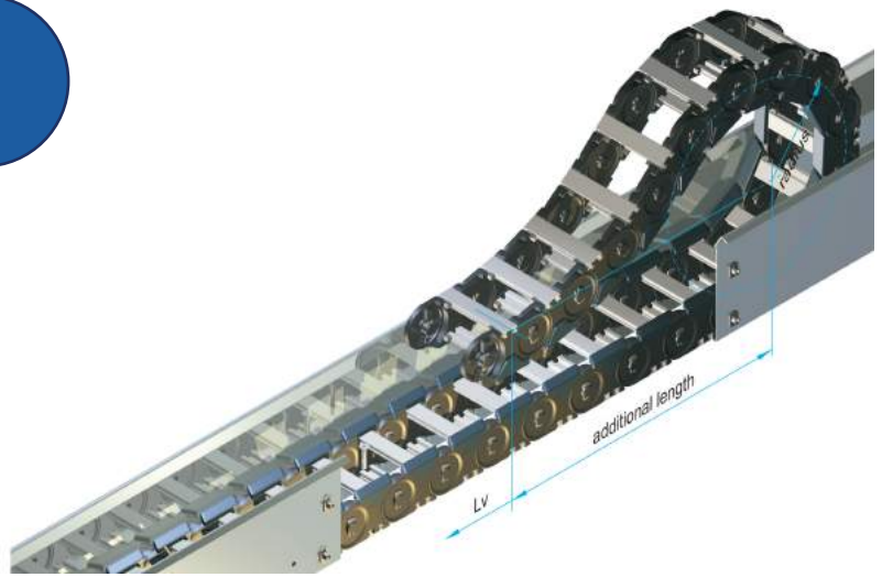
E -200 System - PLE Cable Chain with 2 section guide trough.
